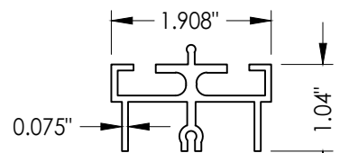
41 SUB-SILL TRACK SUPPORT
