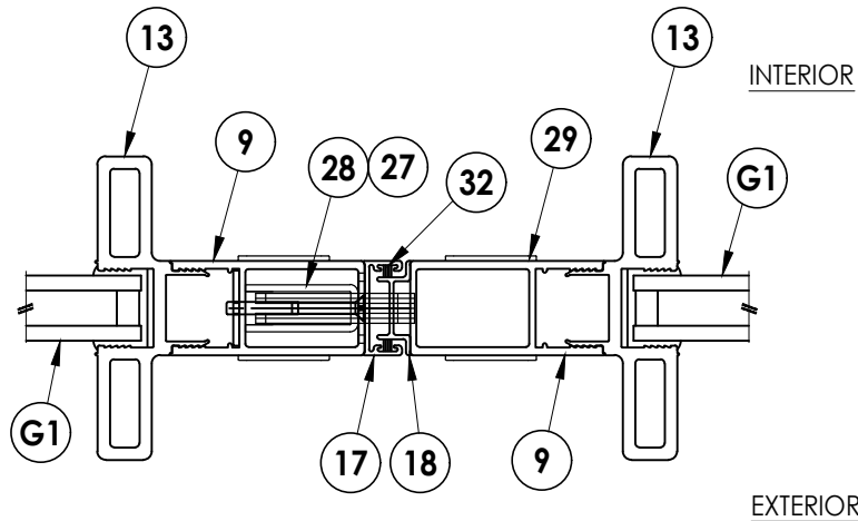
2 3 HORIZONTAL CROSS SECTION
