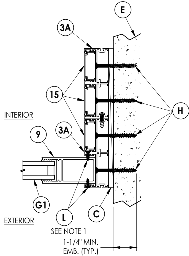
3 3 HORIZONTAL CROSS SECTION Direct to masonry
