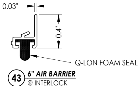
6" AIR BARRIER MOUNTED @ TOP & BOTTOM OF EXTERIOR INTERLOCK STILE
